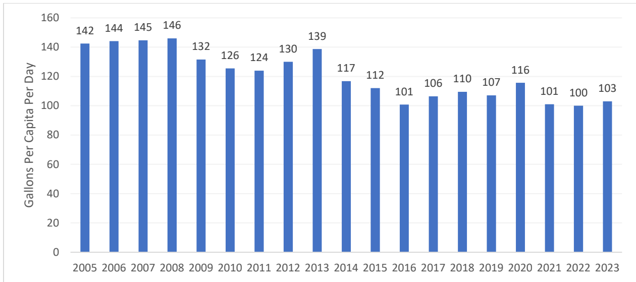
FIGURE 9: MARIN WATER PER CAPITA WATER USE
