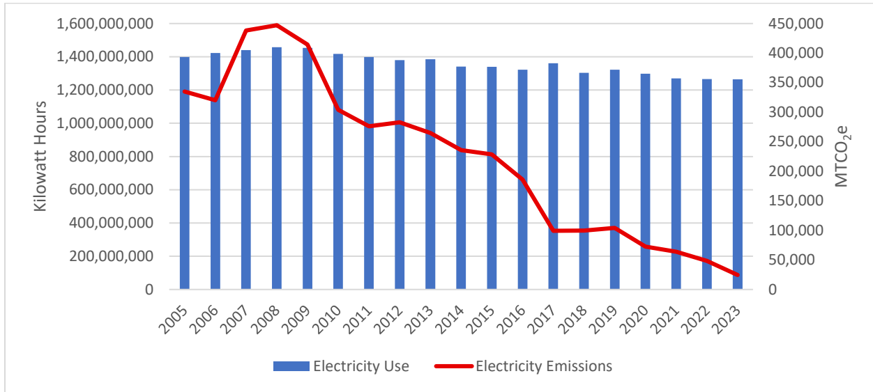
FIGURE 4: ELECTRICITY CONSUMPTION AND EMISSIONS
