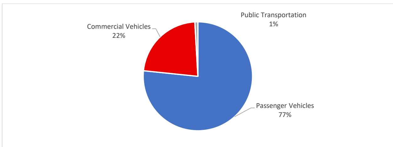
FIGURE 7: TRANSPORTATION EMISSIONS BY VEHICLE CATEGORY, 2023
