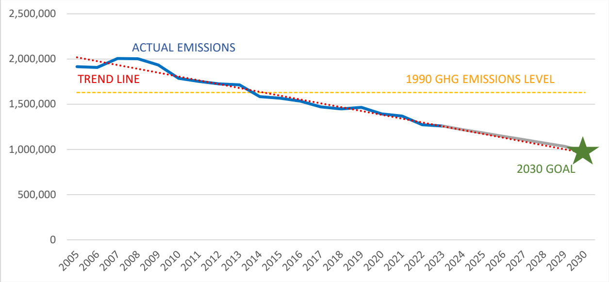
FIGURE 1: MARIN COUNTY GREENHOUSE GAS EMISSIONS AND TARGETS
