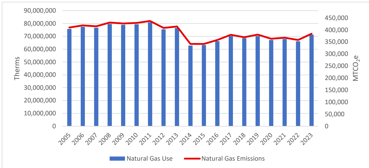
FIGURE 5: NATURAL GAS CONSUMPTION AND EMISSIONS
