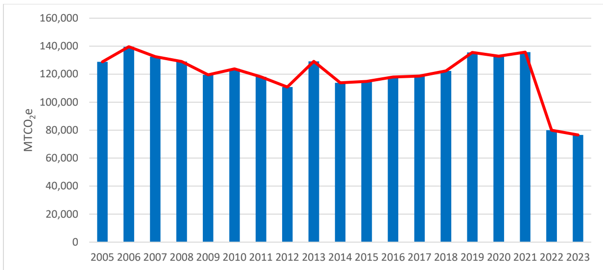
FIGURE 11: AGRICULTURE EMISSIONS
