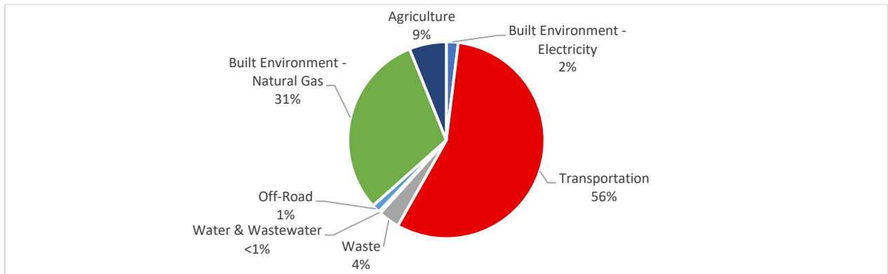
FIGURE 2: EMISSIONS BY SECTOR, 2023
